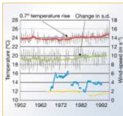
Figure 1 Historical monthly weather records for Lake Tanganyika. Temperature data: red line, Bujumbura; green line, Mbala (gaussian average over six years); grey lines, monthly temperatures. Wind-speed data: blue squares, Mbala; yellow dots, Bujumbura (gaussian average over two years). Created with original O'Reilly et al. weather data.
